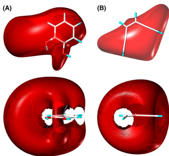
Figure 1. Isopotential surfaces of the catechol fragment ( A ) of dopamine and the endiyn core unit ( B ) of the non-aromatic dopamine receptor agonist FAUC 88 contouring negative electrostatic potentials ( -1 kcal/mol) viewed from the front side (top) and from the bottom side (below).
