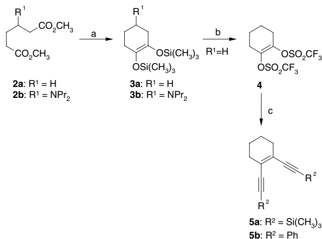
Scheme 1. Reagents and conditions: (a) Na, chlorotrimethylsilane, toluene, for 2a : rt, 1.5 h, 82%; for 2b : rt, 5 h, rt, 30 min, 61%; (b) (1) MeLi, DME, -60^{\circ}\text{C} to -20^{\circ}\text{C} , 2 h; (2) Tf 2 O, -78^{\circ}\text{C} to 10^{\circ}\text{C} , 15 h; (c) trimethylsilylacetylene for 5a , phenylacetylene for 5b , Pd(PPh 3 ) 4 , CuI, EtMe 2 N, THF, rt, for 5a : 3 h, 50%; for 5b : 10 h, 65%.
