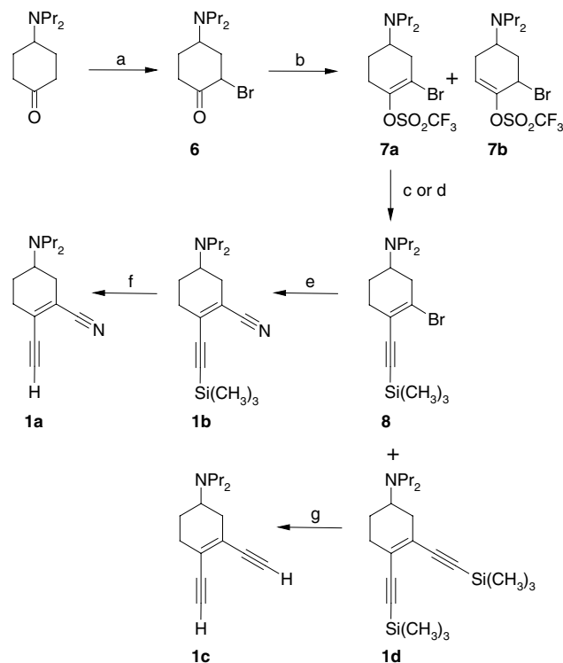
Scheme 2. Reagents and conditions: (a) (1) LDA, THF, -78^{\circ}\text{C} , 1 h; (2) dibromotetrachloroethane, THF, -90^{\circ}\text{C} , 30 min, 66%; (b) (1) LiHMDS, THF, -78^{\circ}\text{C} , 1.75 h; (2) 2-[N,N-bis-(trifluoromethylsulfonyl)-amino]-5-chloropyridine, THF, -78^{\circ}\text{C} to -20^{\circ}\text{C} , 2.25 h, rt, 1 h, 36% 7a , 15% 7b ; (c) trimethylsilylacetylene, Pd(PPh 3 ) 4 , CuI, piperidine, THF, 40^{\circ}\text{C} , 3.5 h, 67% 8 ; 7% 1d ; (d) trimethylsilylacetylene, Pd(PPh 3 ) 4 , CuI, piperidine, THF, 95^{\circ}\text{C} , 1 h, 24% 8 , 42% 1d ; (e) CuCN, Pd 2 (dba) 3 , dppf, dioxane, reflux, 2.75 h, 54%; (f) Bu 4 NF, THF, -20^{\circ}\text{C} , 45 min, 60%; (g) Bu 4 NF, THF, -20^{\circ}\text{C} , 20 min, 82%.
